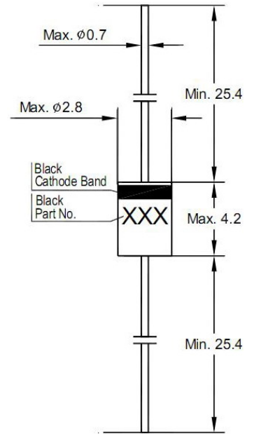
Glass Case DO-41 Dimensions in mm
